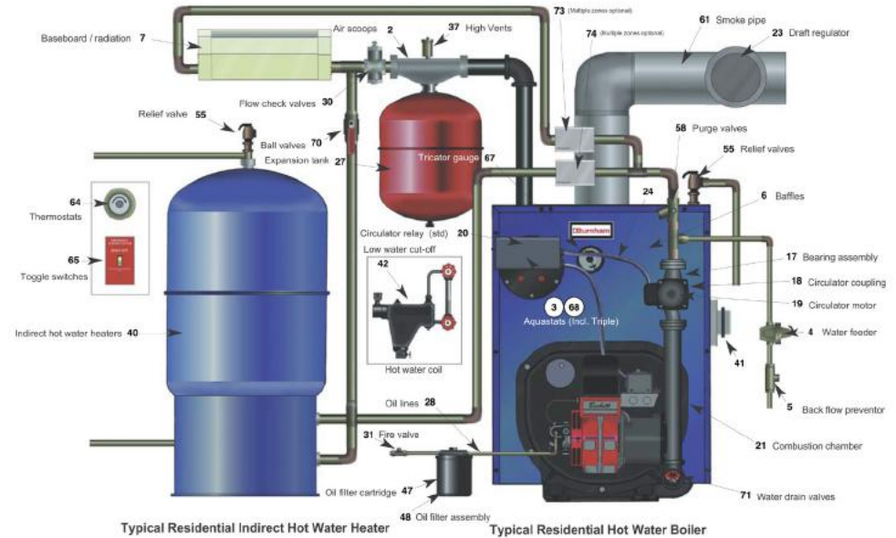
Typical Residential Indirect Hot Water Heater Typical Residential Hot Water Boiler
