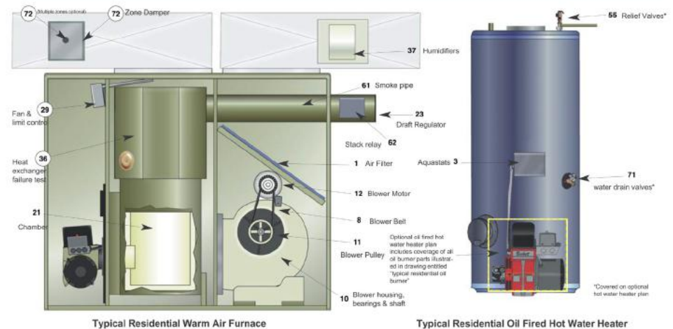
Typical Residential Warm Air Furnace
