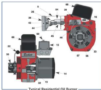
Typical Residential Oil Burner
